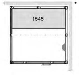
PANACEA STEAM 1717 Size: 1725 x 1725 mm Item no. 9607 5070
