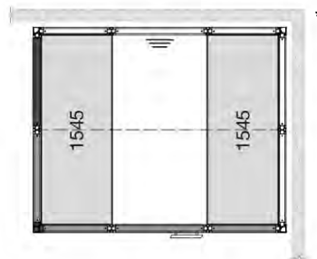
PANACEA STEAM 2117 Size: 2125 x 1725 mm Item no. 9607 5076
